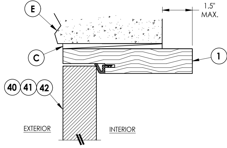
4 6 VERTICAL CROSS SECTION Shown Direct to Masonry w/ 6-9/16" jamb
