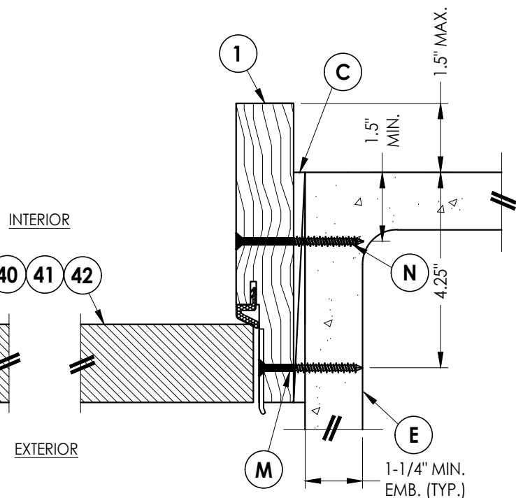
6 6 HORIZONTAL CROSS SECTION Shown Direct to Masonry w/ 6-9/16" jamb
