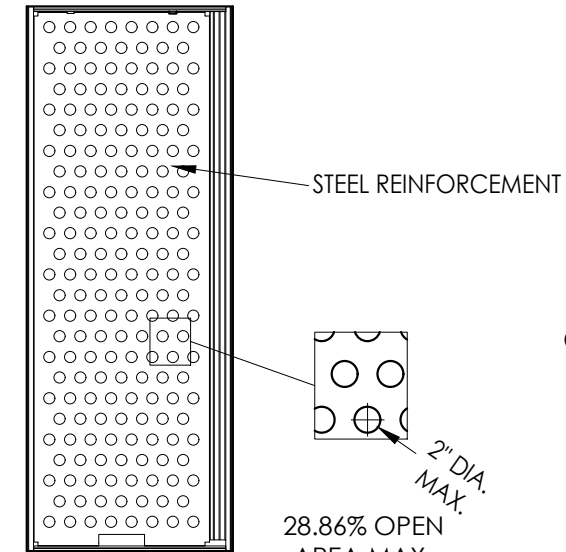
DETAIL A-A PANEL REINFORCEMENT (0.023\"
